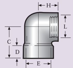
90° Adapter Elbow
