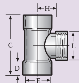
Adapter Tee
