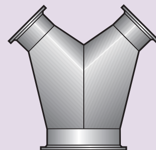
Double Y Branch
